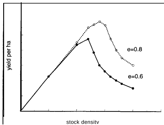
Figure 1: Effect of a theoretical increase in nitrogen fixation efficiency in white clover on the relationship between stock density and yield of animal product per hectare as predicted by a model of soil/plant/animal interaction (Schwinning & Parsons 1996a; 1996b). Nitrogen fixation is assumed to be either 60% ( e=0.60 ) or 80% ( e=0.8 ) as efficient as mineral N uptake, in terms of energy costs of assimilation.
