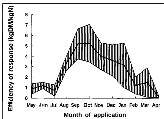
Figure 4: Annual pattern of pasture response to N fertiliser application (3 year average). Shaded area shows SEM (from Roberts & Thomson 1989).
