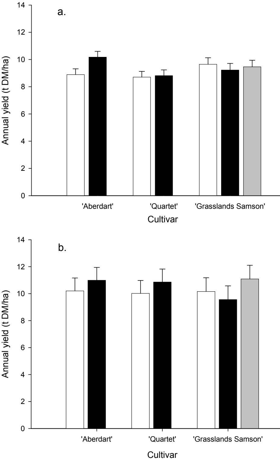
Figure 2 Annual dry matter (DM) yield of three perennial ryegrass cultivars either not infected with endophyte (white), or infected with AR1 (black) or AR37 (grey) endophyte in Year 1 (a) and Year 2 (b).
