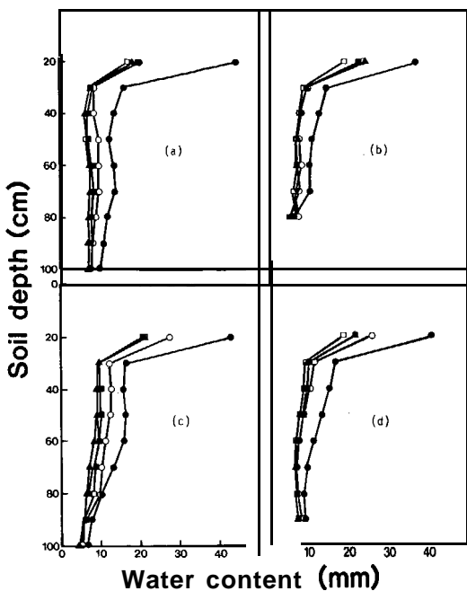
Figure 2 Changes in soil water content under lucerne (a), phalaris (b) lucerne-prairie (c) and lucerne-phalaris (d) swards in deep soils during a drying cycle in spring 1988. (●) 29/9/88, (○) 13/10/88, (■) 22/10/88, (□) 29/10/88, (A) 7/11/88.
